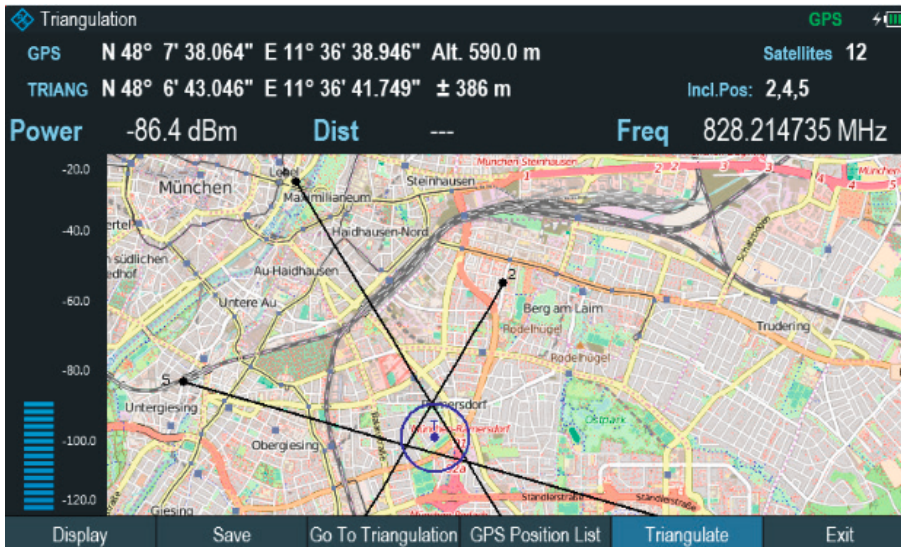
Locating a signal with the R&S®ZPH-K15 interference analysis option with R&S®HE400 series directional antenna
